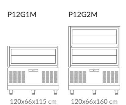
120x66x115 cm 120x66x160 cm
